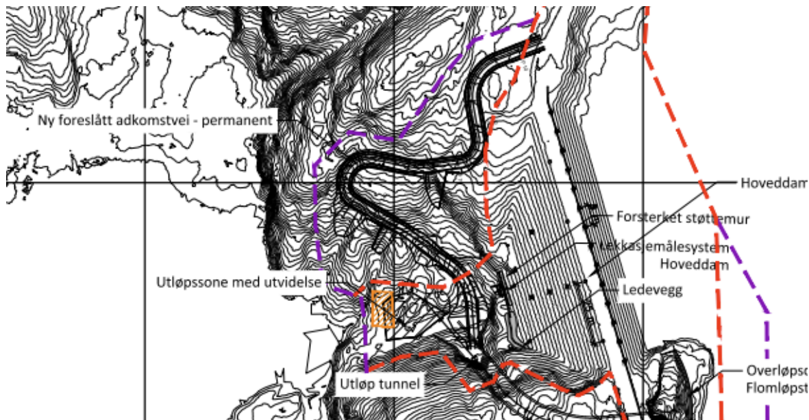
Figur 2: Revidert plan
